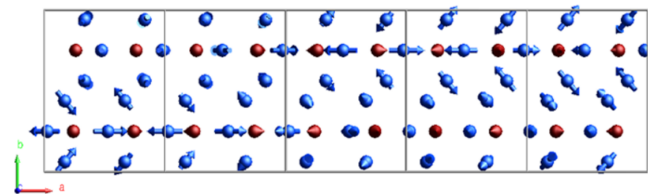
Figure 13 Spin modulation of Ho 3 Co at 18 K for Ho (blue) and Co (red) represented in a 5 × 1 × 1 supercell of the parent orthorhombic unit cell. The modulation of Ho1 and Ho2 is described as fanlike, with a fan spanning of 100°. The fan plane of the Ho1 is parallel to (101), whereas Ho2 spins are at an angle of 57° away from the a axis. The modulation of the Co spins is a circular cycloidal restricted to be parallel to (101).
