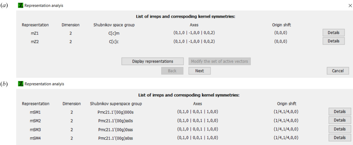
Figure 5 First informative window after representation analysis for a (a) parent space group Cmc2m and \mathbf{k} = (00\frac{1}{2}) and (b) parent space group Pnma and \mathbf{k} = (\alpha 00) . It lists the minimal symmetry groups (kernels) for the correspondent irreps. The lateral button ‘Details’ displays the symmetry operators for the kernel space group (a) or superspace group (b) of the irrep and the respective transformation to the standard setting. The irrep matrices can be consulted in ‘Display representations’ at the bottom.
