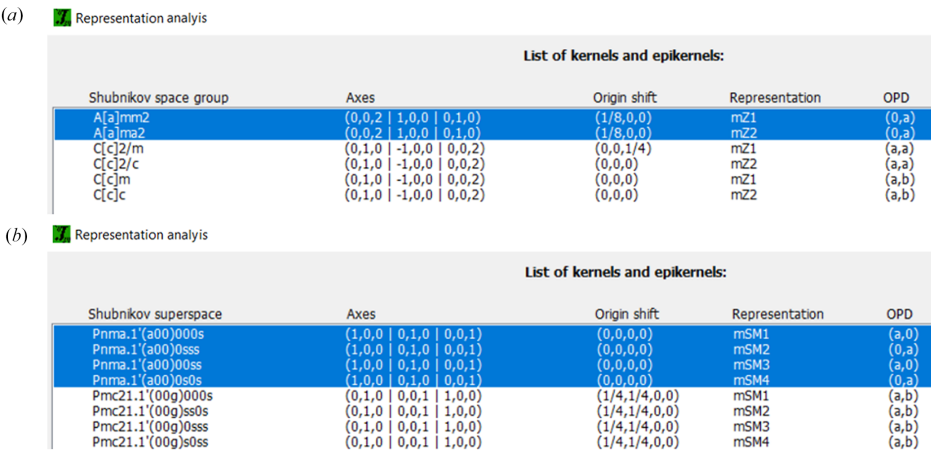
Figure 6 Second representation analysis window listing the isotropy subgroups associated with the irreps and respective order parameter directions (OPD) for structures (a) commensurate and (b) incommensurate from Fig. 5.
