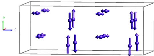
Figure 12 The magnetic structure of Dy 2 Co 3 Al 9 at 2 K is described in the non-centrosymmetric MSG A u mm2 . The structure consists of alternating layers of moments oriented parallel to (110) and moments along [001]. Only the Dy atoms are represented in the unit cell.
