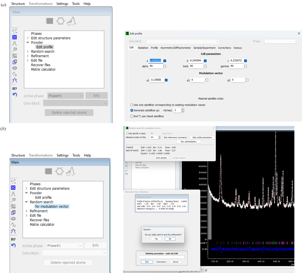
Figure 10 Sequence to make a random search for the k vector for powder data.
